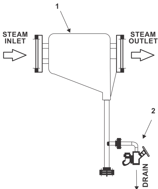
Figure3: Typical Installation of FMSEP54 on a steam line
