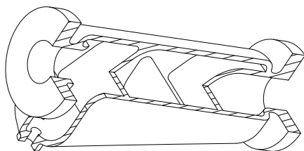
Figure 1: Forbes Marshall Moisture Separator - Flanged
