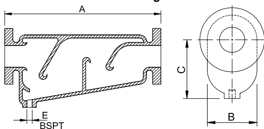
Figure 2: Dimensional drawing of FMSEP54
