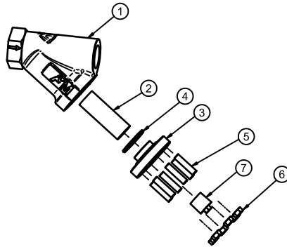
Figure 5 : Exploded view of Forbes Marshall Forged Strainer [FMSTR51#600/FMSTR52#600]
