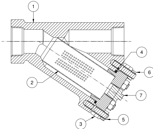
Figure 1 : Forbes Marshall Forged Strainer
