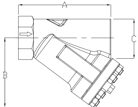
Figure 2 : Dimensional Drawing of FMSTR51#600 / FMSTR52#600
