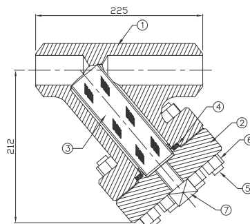
Figure 1: FMSTR72 in butt weld end connection
