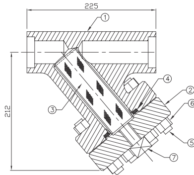
Figure 2: FMSTR72 in socket weld end connection
