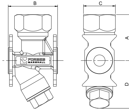
Figure 2: Dimensional drawing of FMTD64-S
