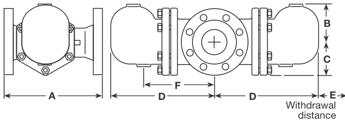
Figure 2: Dimensional Drawing of SOFT53-X
