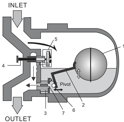
3(a) Trap Discharge Open
