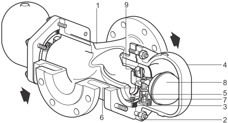
Figure: 1 Single Orifice Float Tap with TV
