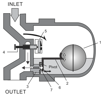
3(b) Trap Discharge Closed
