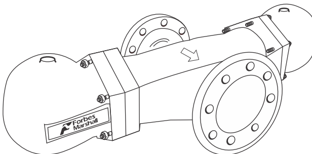
Figure 5: Cover casting with the arrow
